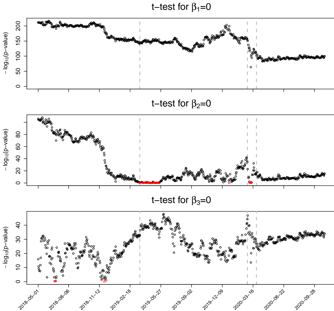
Figure A5: P-values in Nelson and Siegel (1987) model. P-values of t-tests for \beta_{j,t} = 0 , j = 1, 2, 3 in Nelson and Siegel (1987) model. Red points correspond to non-significant coefficients ( p\text{-value} > 0.05 ). The vertical gray dashed lines show our subdivision in periods.
