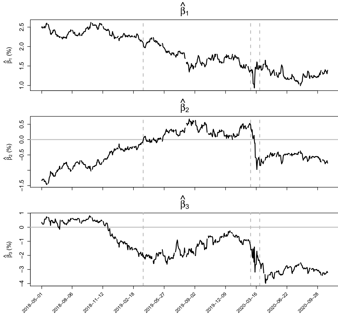
Figure 6: Time series of estimated \hat{\beta}_{1,t} , \hat{\beta}_{2,t} and \hat{\beta}_{3,t} in the Nelson and Siegel (1987) model (with \lambda_t = 0.0609 ). The vertical gray dashed lines show our subdivision in periods. All values are in percentage.
